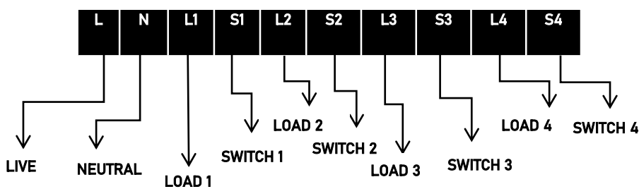
WIRING DIAGRAM
