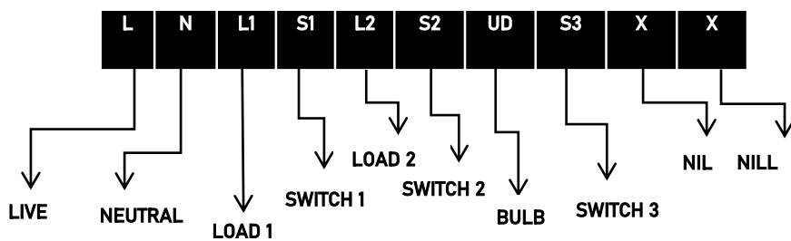
WIRING DIAGRAM
