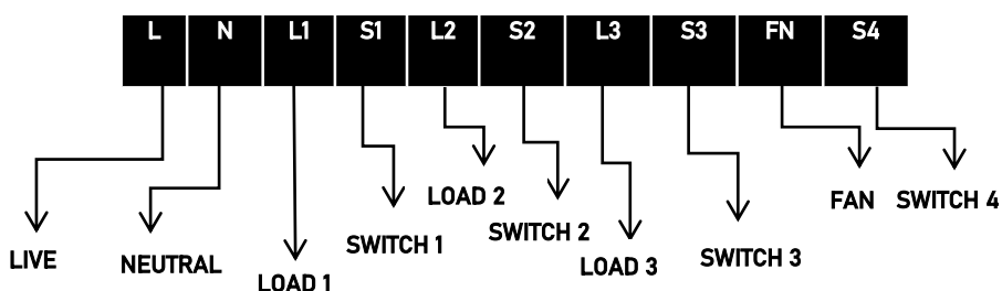
WIRING DIAGRAM
