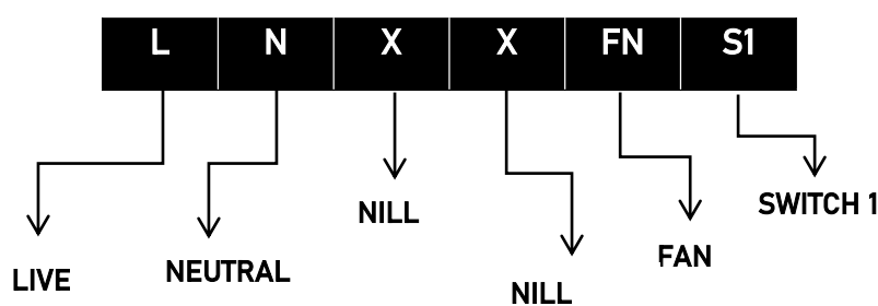
WIRING DIAGRAM
