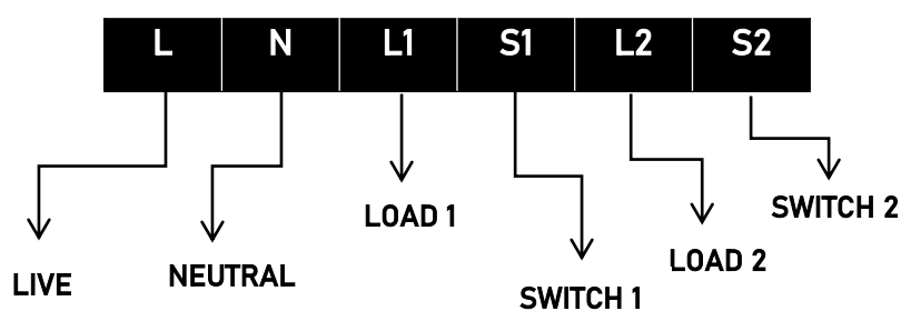
WIRING DIAGRAM
